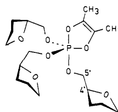
Figure 6. Model compound 6, dominant \text{C}_4\text{-C}_5 , rotamers are drawn for the tetrahydrofurfuryl ligands.
