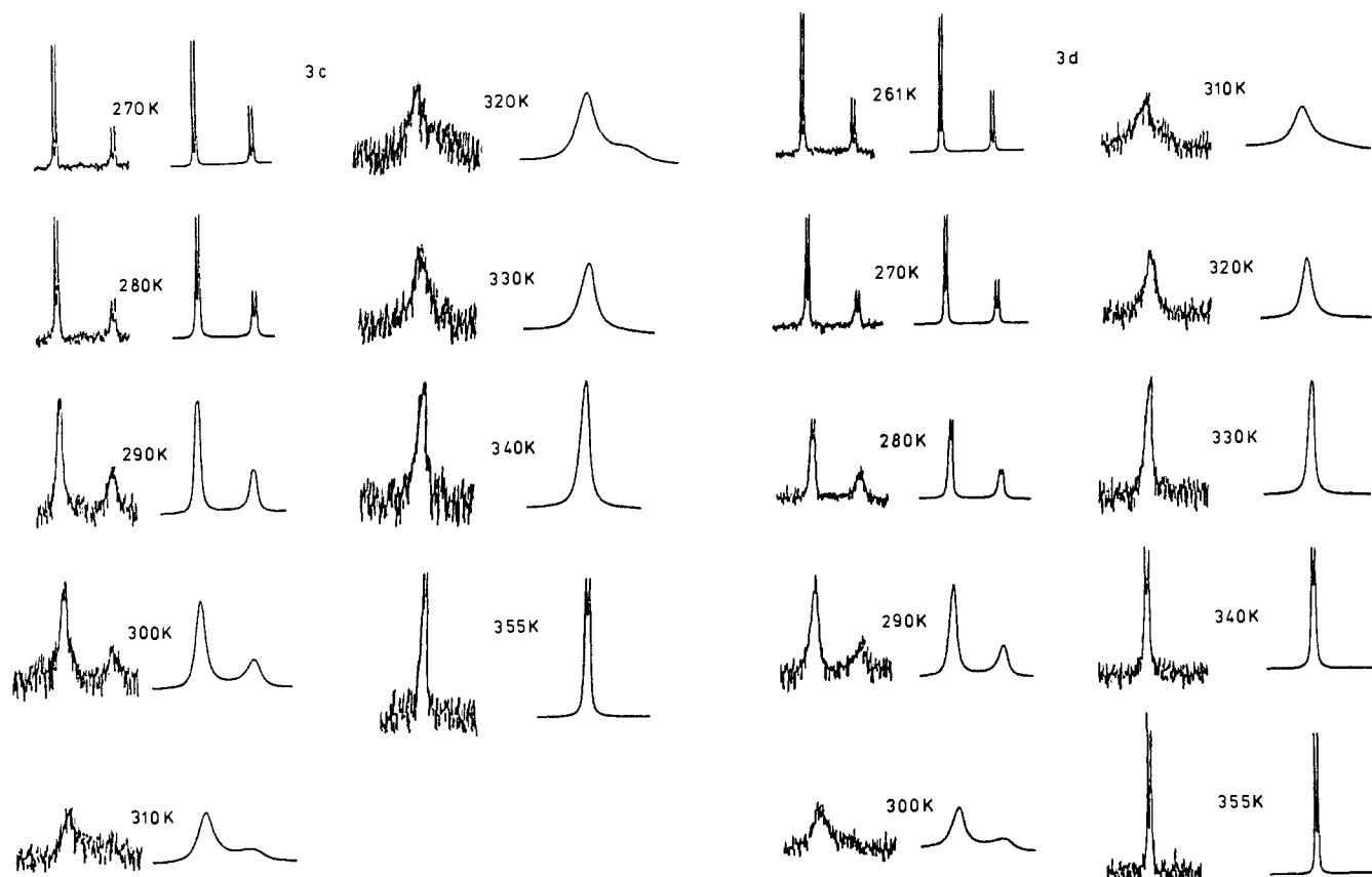
Figure 2. Temperature dependence of the ^{13}\text{C} NMR spectra of the phosphoranones 3c and 3d . Exchange of the oxamethylene carbons. Experimental (left) and calculated (right) spectra at different temperatures.
